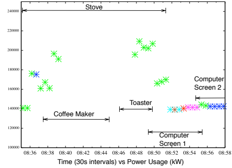
Figure 7. An example of the same power segments from Figure 6, but at a 30 second logging granularity.
