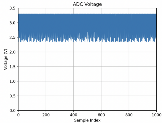
Fig. 5. IEMI ON, tight coupling.
